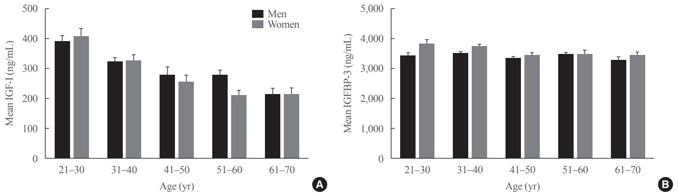
Supplemental Fig. S1. Graph presents the mean \pm standard deviation of (A) insulin-like growth factor-I (IGF-I) and (B) insulin-like growth factor binding protein-3 (IGFBP-3) by 10-year intervals of age group in males (black bar) and females (gray bar).
