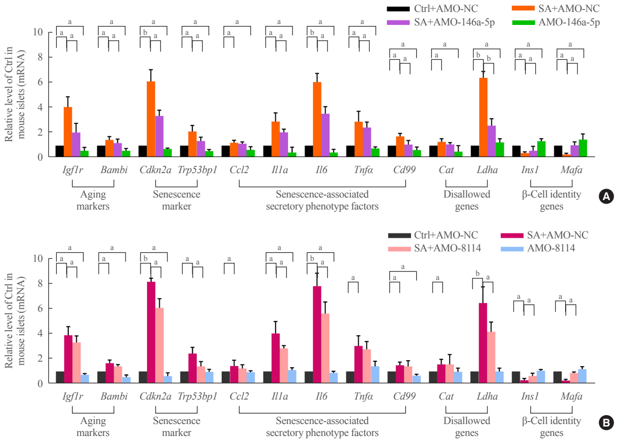
Supplemental Fig. S5. (A, B) Change in the expression of senescence-related genes after silencing of miR-146a-5p and miR-8114 in stearic acid (SA)-treated mouse islets. Each experiment was repeated independently three times. Ctrl, control; AMO, anti-miRNA oligonucleotides; NC, negative control. a P < 0.05 ; b P < 0.01 .
